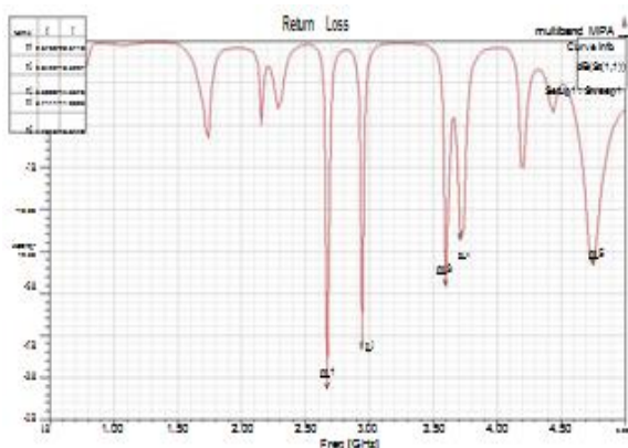
Fig 3: Return loss
