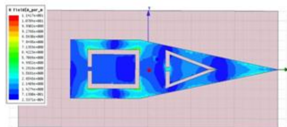
Fig 9: H-field Distributions
