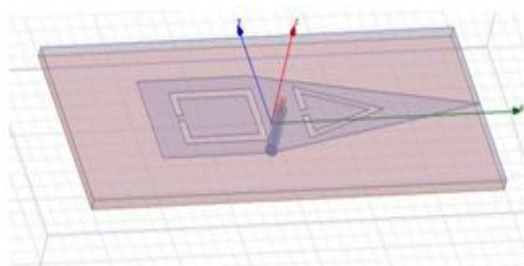
Fig 2: Antenna model
