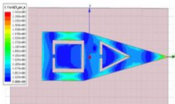
Fig 8: E-field Distributions
