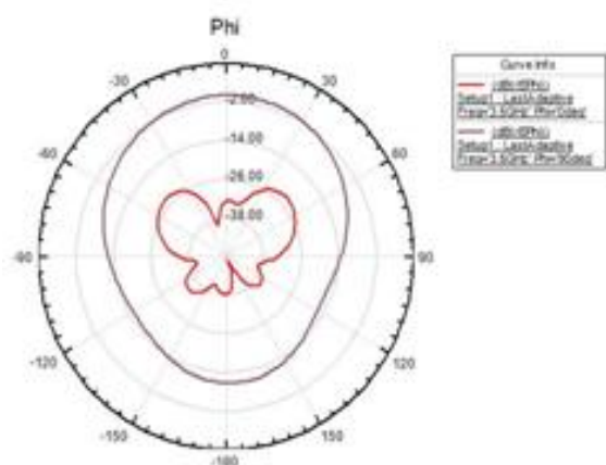
Fig 6: Gain along Phi
