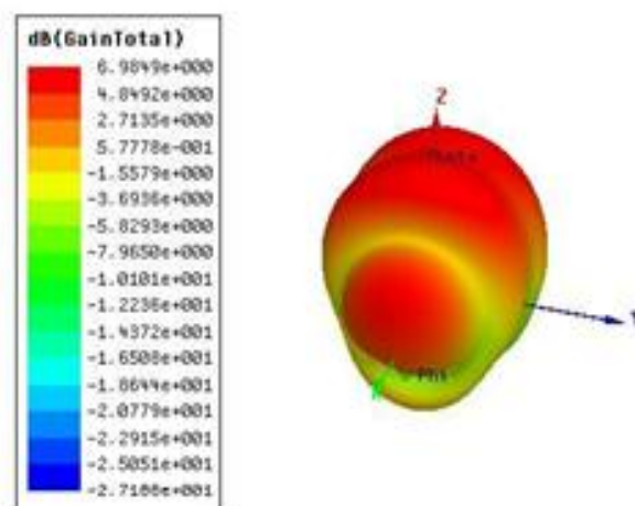
Fig 5: 3D- Gain Total
