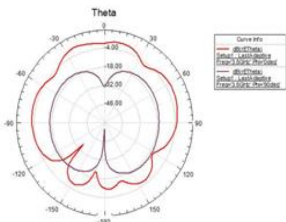
Fig 7: Gain along Theta
